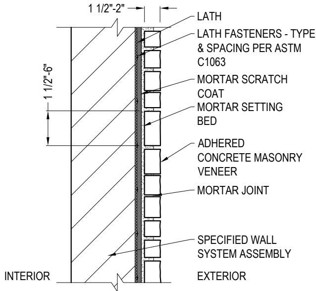
TYPICAL SECTION
