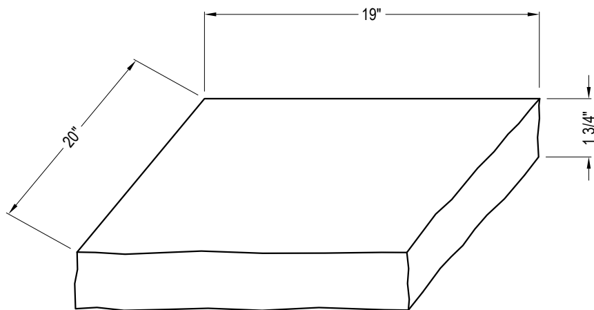
PERSPECTIVE-HEARTHSTONE
